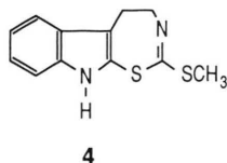
1 , Cyclobassinin 2 , Brassilexin 3 , 5-methoxybrassilexin 4 , Homocyclobassinin
